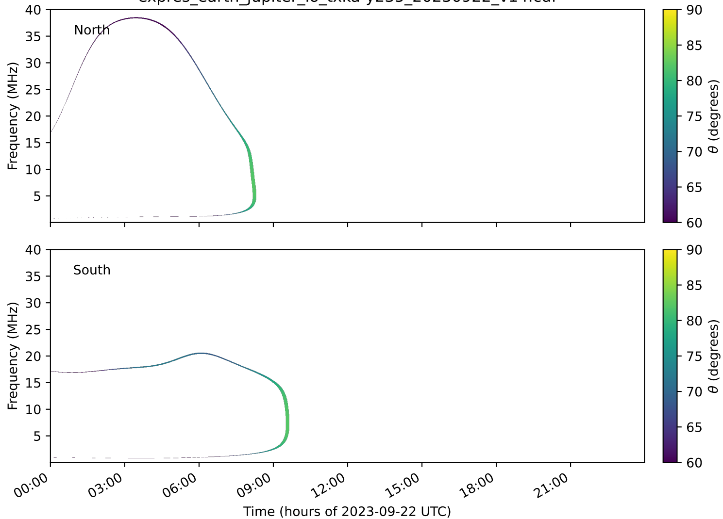
expres_earth_jupiter_io_txka-y235_20230922_v14.cdf
