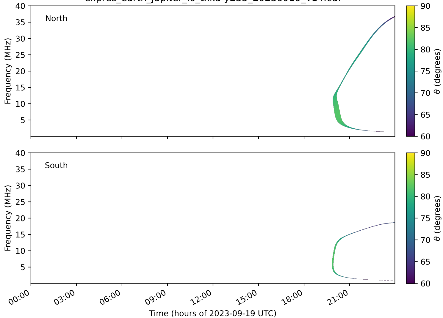
expres_earth_jupiter_io_txka-y235_20230919_v14.cdf
