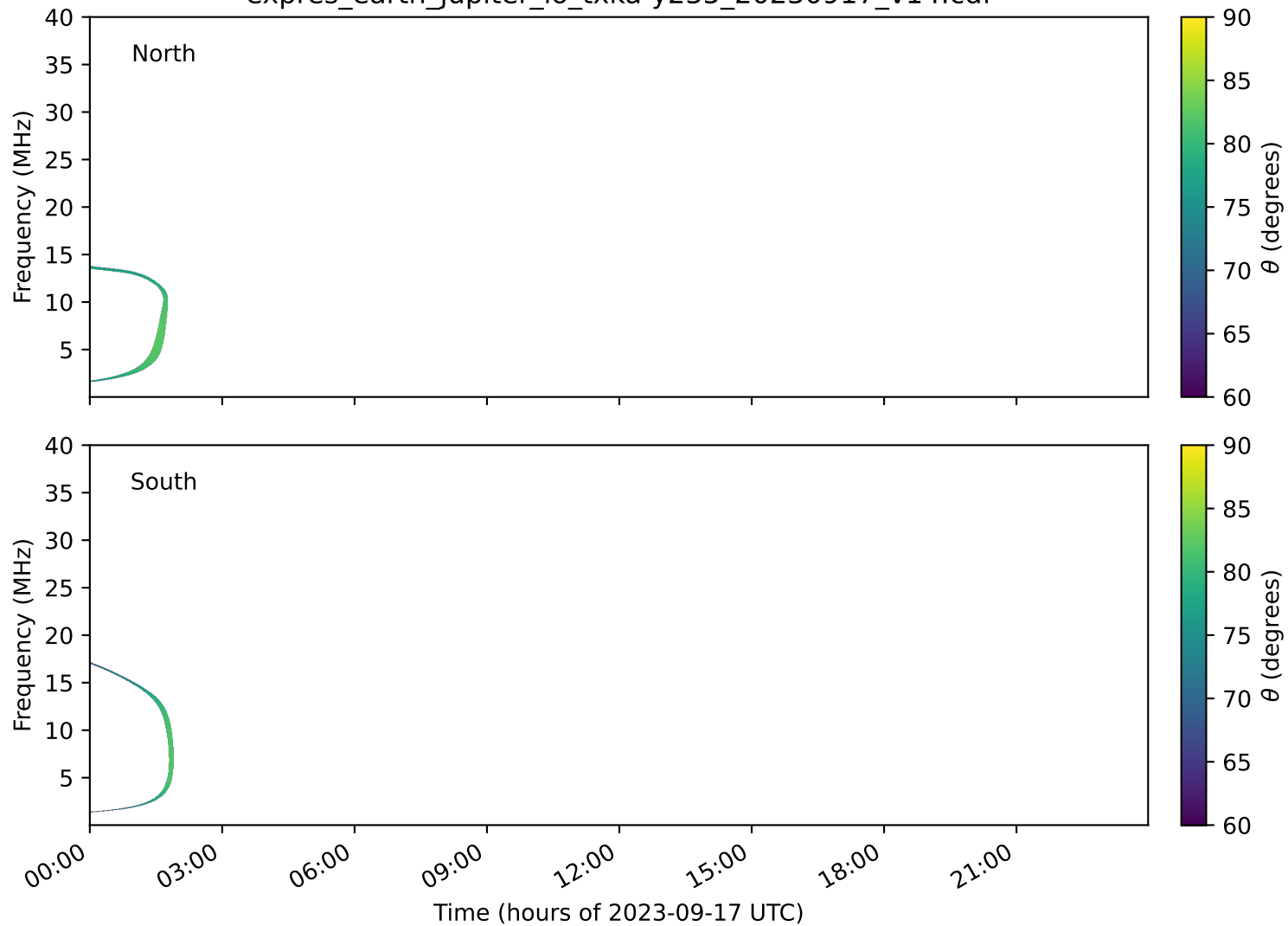
expres_earth_jupiter_io_txka-y235_20230917_v14.cdf
