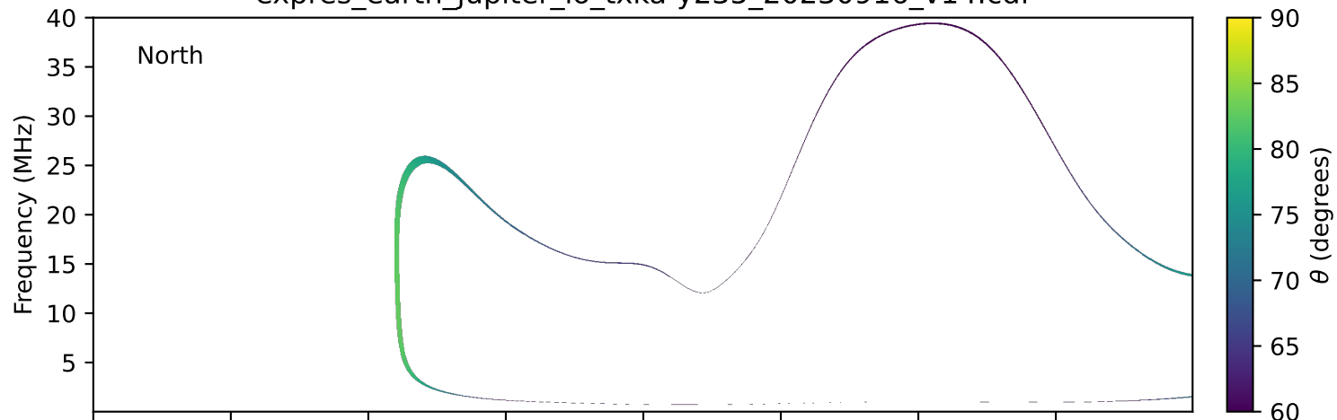
expres_earth_jupiter_io_txka-y235_20230916_v14.cdf
