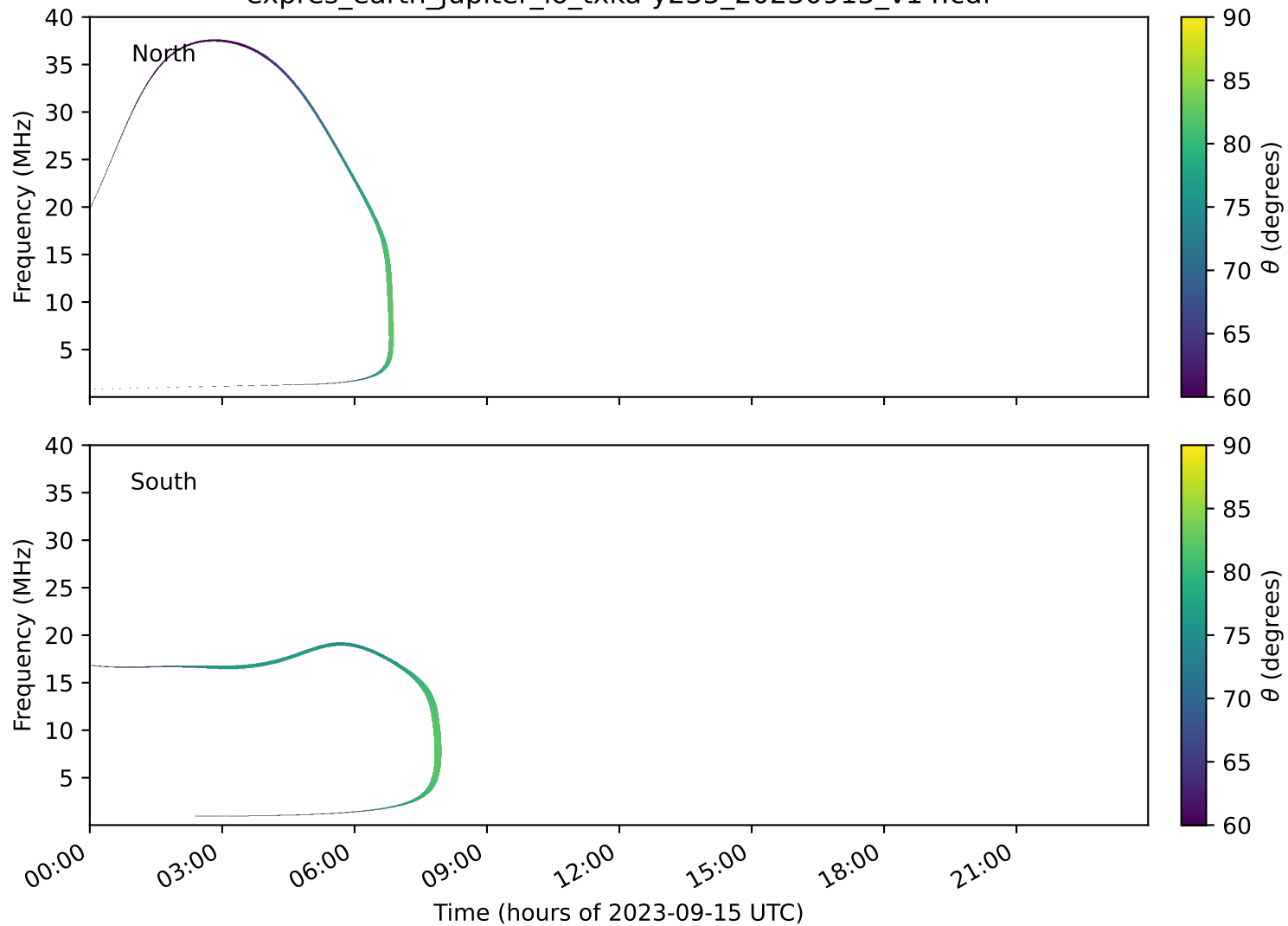
expres_earth_jupiter_io_txka-y235_20230915_v14.cdf
