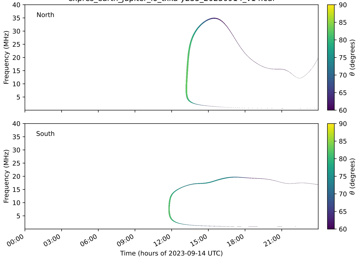
expres_earth_jupiter_io_txka-y235_20230914_v14.cdf
