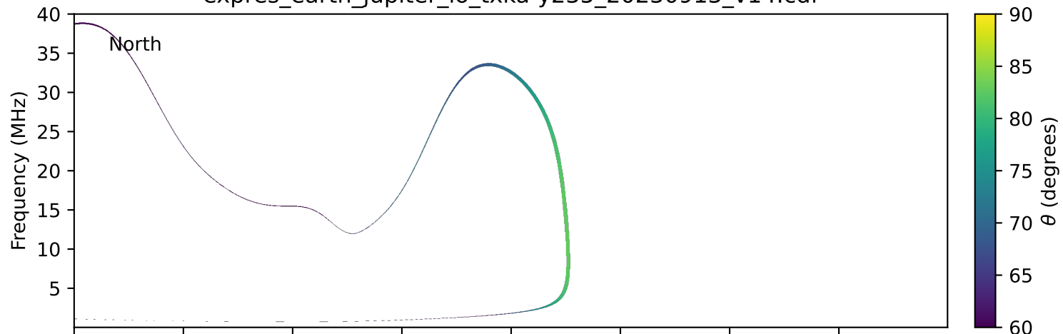
expres_earth_jupiter_io_txka-y235_20230913_v14.cdf
