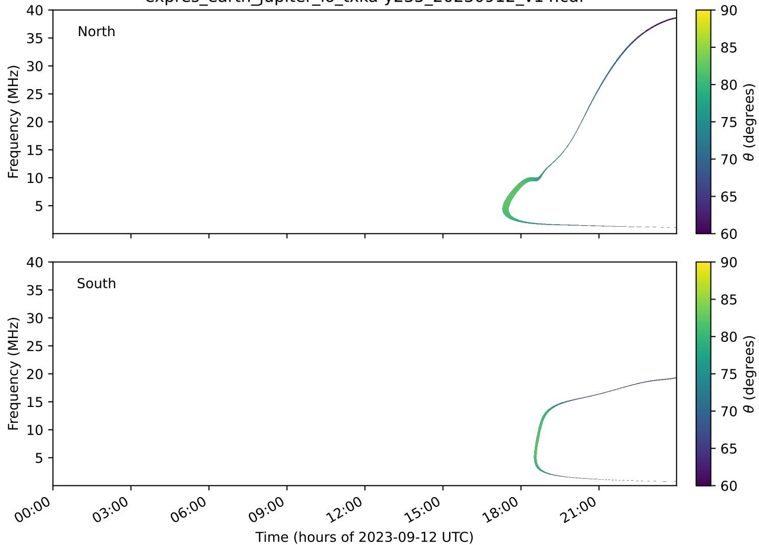
expres_earth_jupiter_io_txka-y235_20230912_v14.cdf
