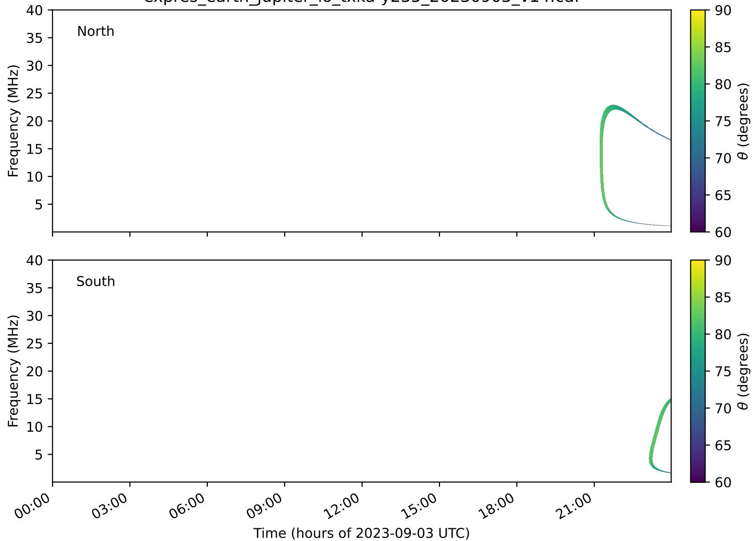
expres_earth_jupiter_io_txka-y235_20230903_v14.cdf
