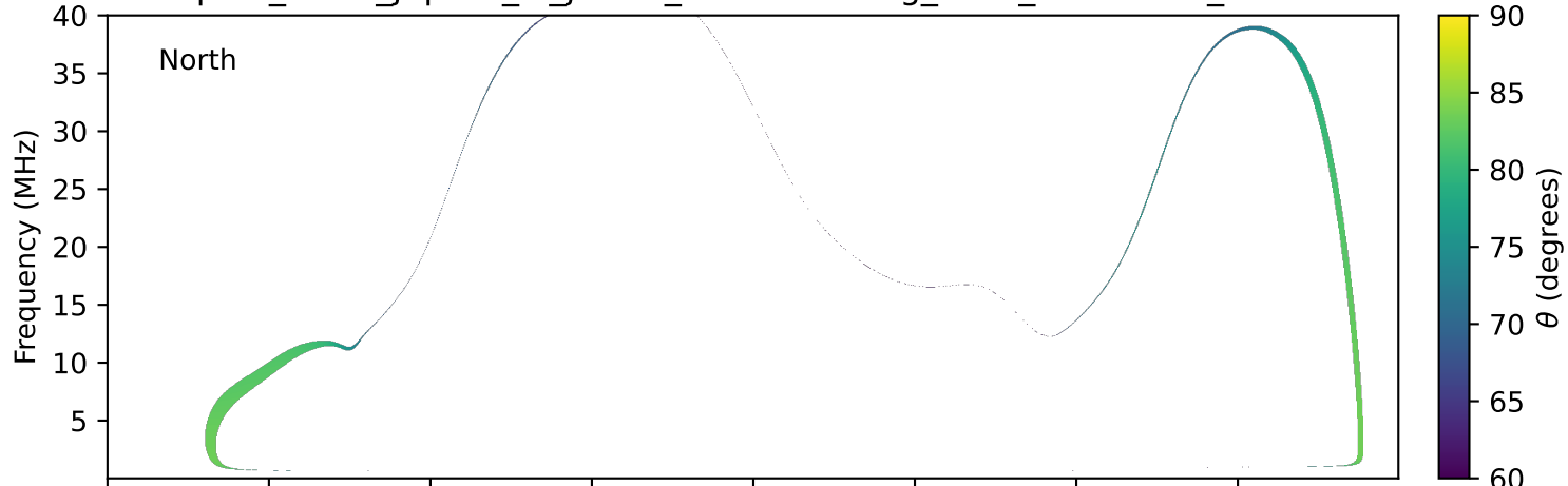
expres_earth_jupiter_io_jrm33_lossc-wid1deg_3kev_20230925_v11.cdf
