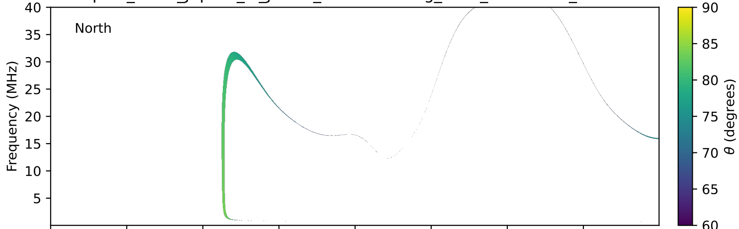
expres_earth_jupiter_io_jrm33_lossc-wid1deg_3kev_20230916_v11.cdf
