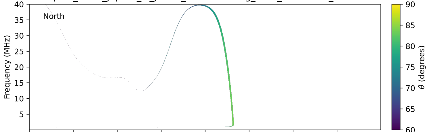
expres_earth_jupiter_io_jrm33_lossc-wid1deg_3kev_20230913_v11.cdf
