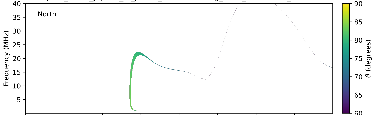
expres_earth_jupiter_io_jrm09_lossc-wid1deg_3kev_20230923_v11.cdf
