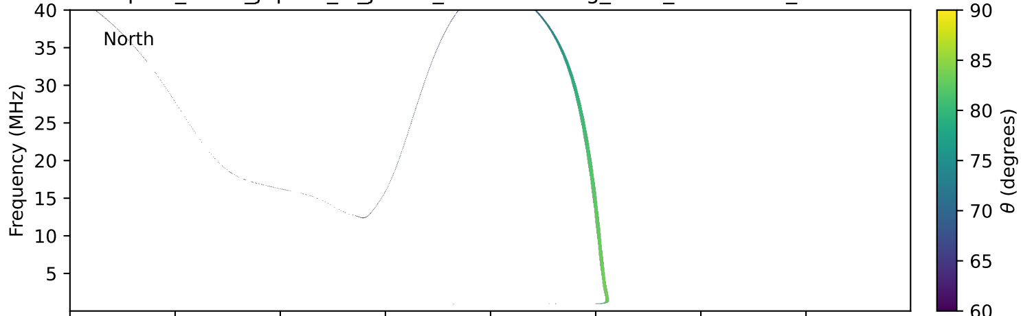
expres_earth_jupiter_io_jrm09_lossc-wid1deg_3kev_20230920_v11.cdf
