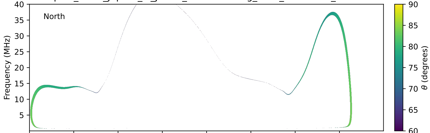
expres_earth_jupiter_io_jrm09_lossc-wid1deg_3kev_20230918_v11.cdf
