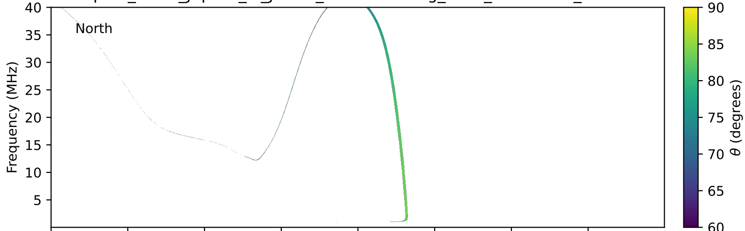
expres_earth_jupiter_io_jrm09_lossc-wid1deg_3kev_20230913_v11.cdf
