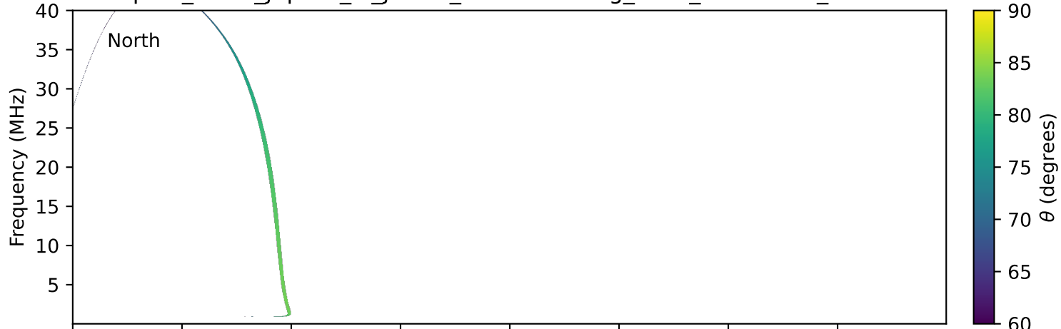
expres_earth_jupiter_io_jrm09_lossc-wid1deg_3kev_20230908_v11.cdf
