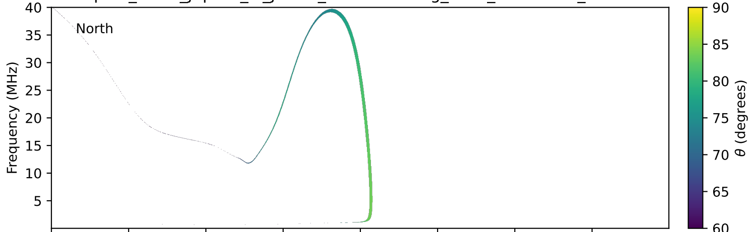
expres_earth_jupiter_io_jrm09_lossc-wid1deg_3kev_20230906_v11.cdf
