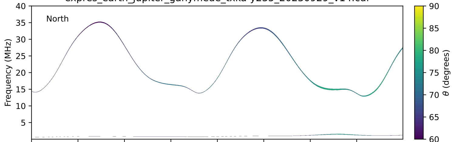
expres_earth_jupiter_ganymede_txka-y235_20230929_v14.cdf
