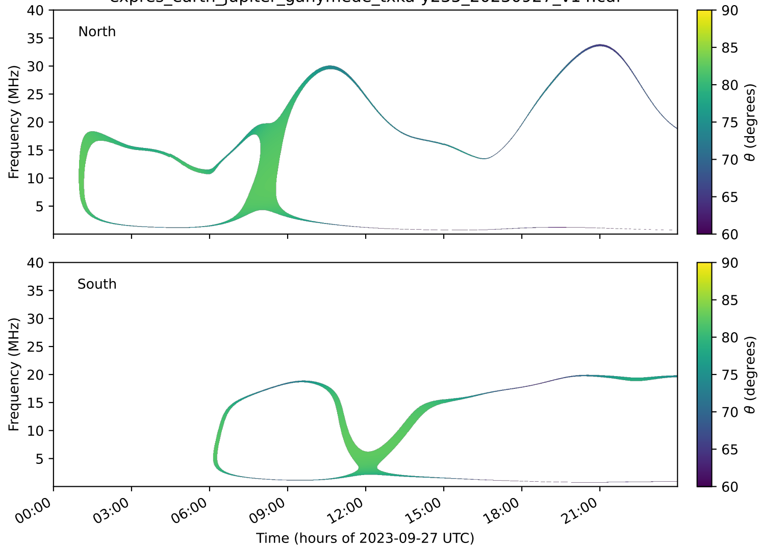
expres_earth_jupiter_ganymede_txka-y235_20230927_v14.cdf
