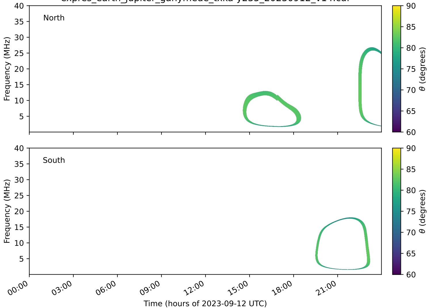
expres_earth_jupiter_ganymede_txka-y235_20230912_v14.cdf
