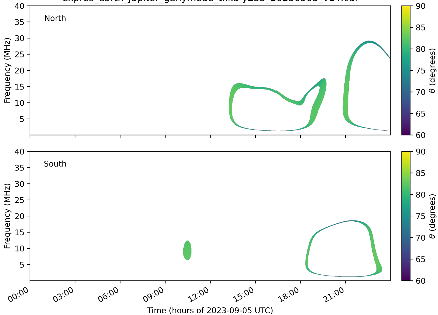
expres_earth_jupiter_ganymede_txka-y235_20230905_v14.cdf
