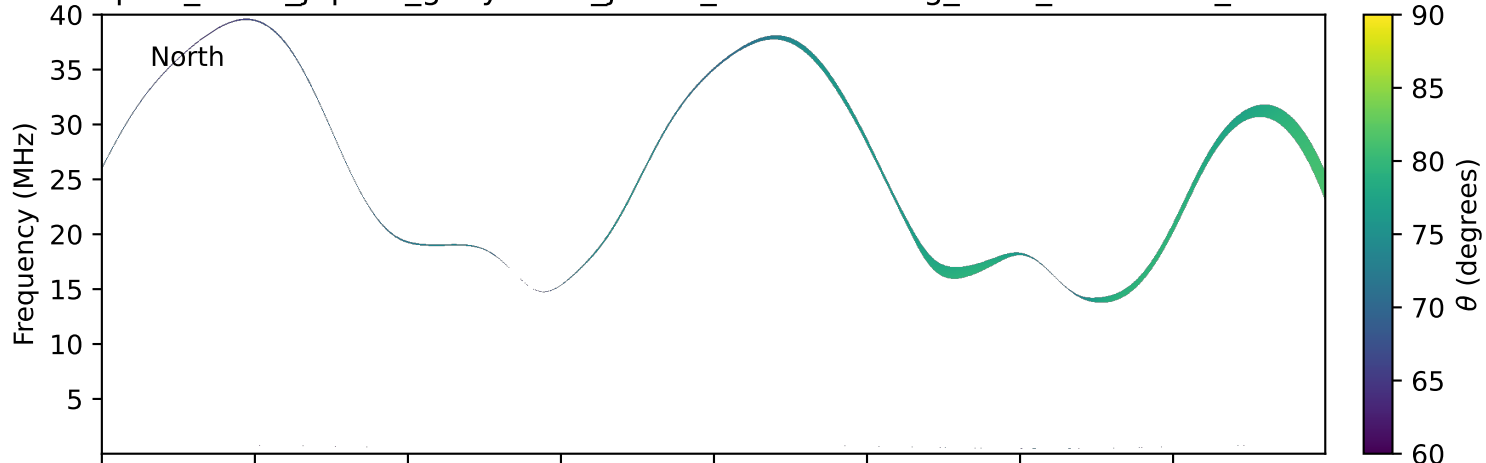
expres_earth_jupiter_ganymede_jrm33_lossc-wid1deg_3kev_20230908_v11.cdf
