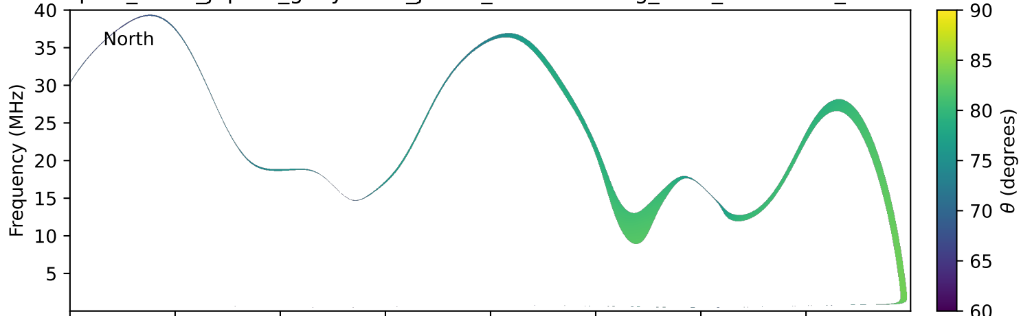
expres_earth_jupiter_ganymede_jrm33_lossc-wid1deg_3kev_20230901_v11.cdf
