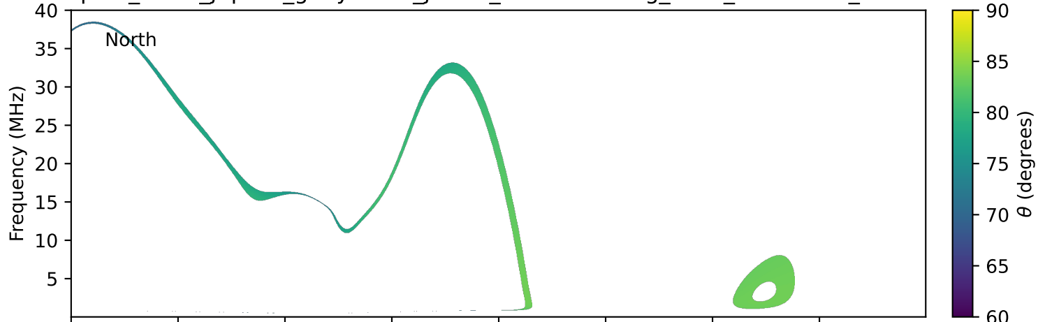
expres_earth_jupiter_ganymede_jrm09_lossc-wid1deg_3kev_20230930_v11.cdf
