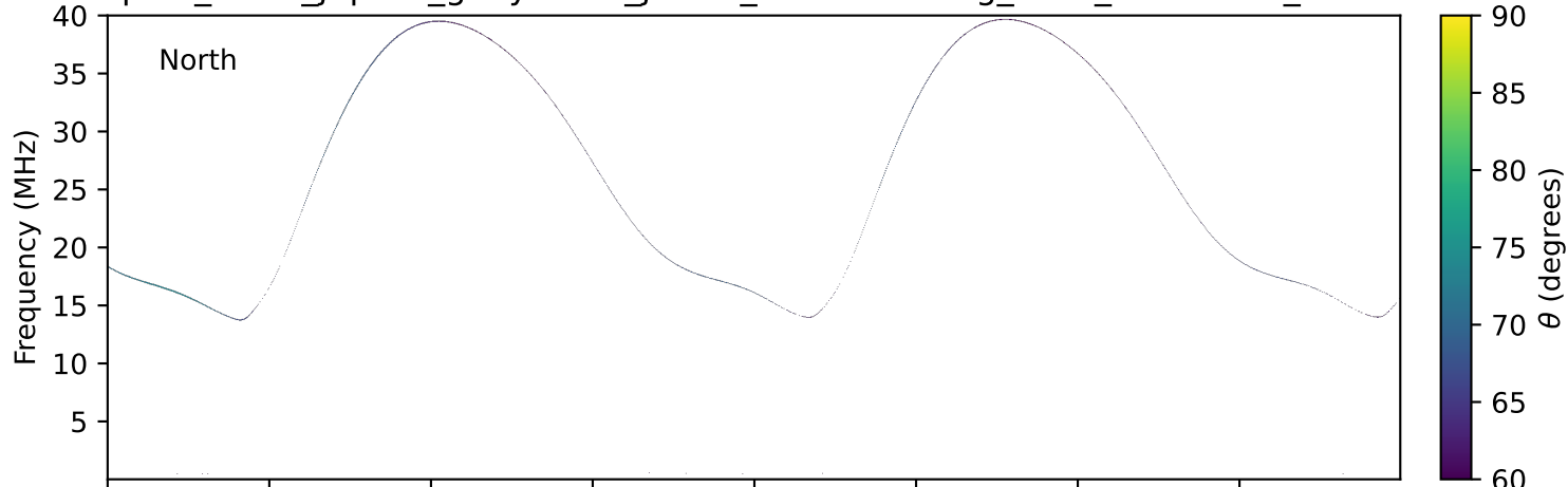
expres_earth_jupiter_ganymede_jrm09_lossc-wid1deg_3kev_20230921_v11.cdf
