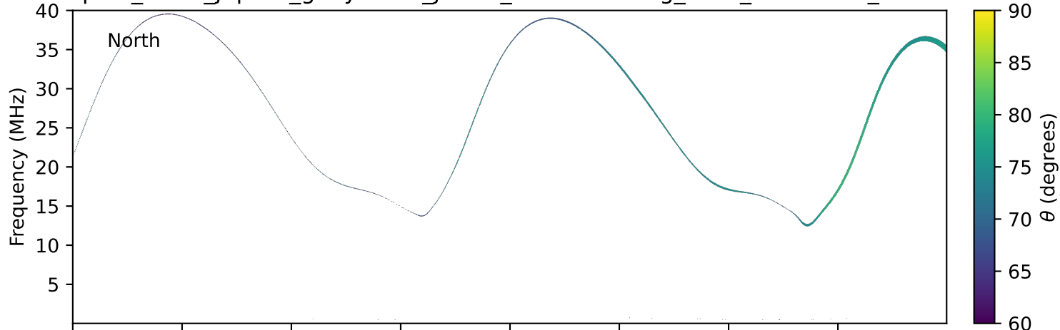
expres_earth_jupiter_ganymede_jrm09_lossc-wid1deg_3kev_20230915_v11.cdf
