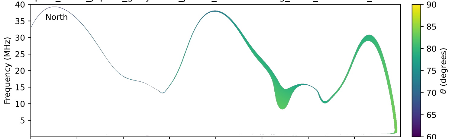
expres_earth_jupiter_ganymede_jrm09_lossc-wid1deg_3kev_20230901_v11.cdf
