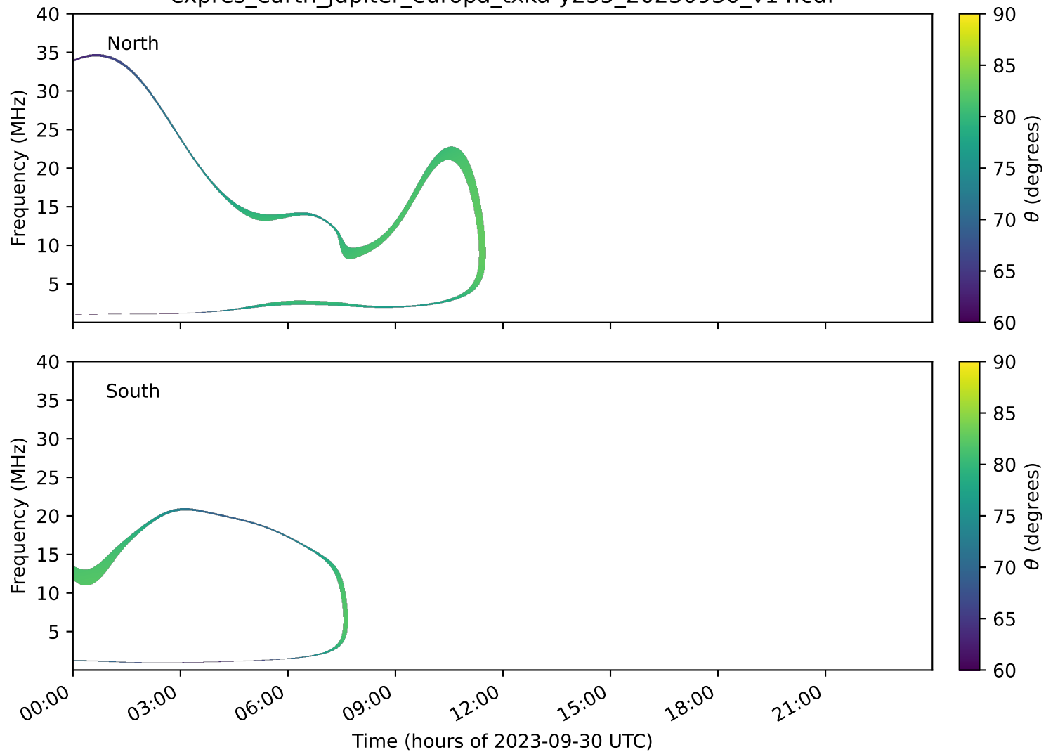
expres_earth_jupiter_europa_txka-y235_20230930_v14.cdf
