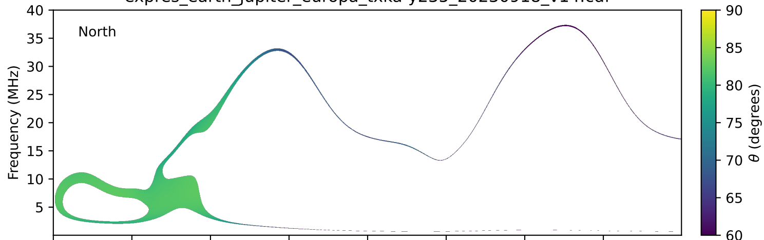
expres_earth_jupiter_europa_txka-y235_20230918_v14.cdf
