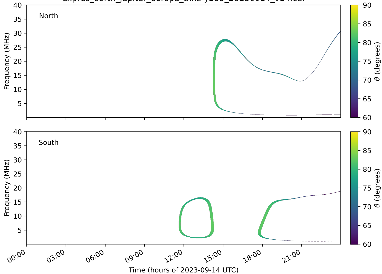
expres_earth_jupiter_europa_txka-y235_20230914_v14.cdf
