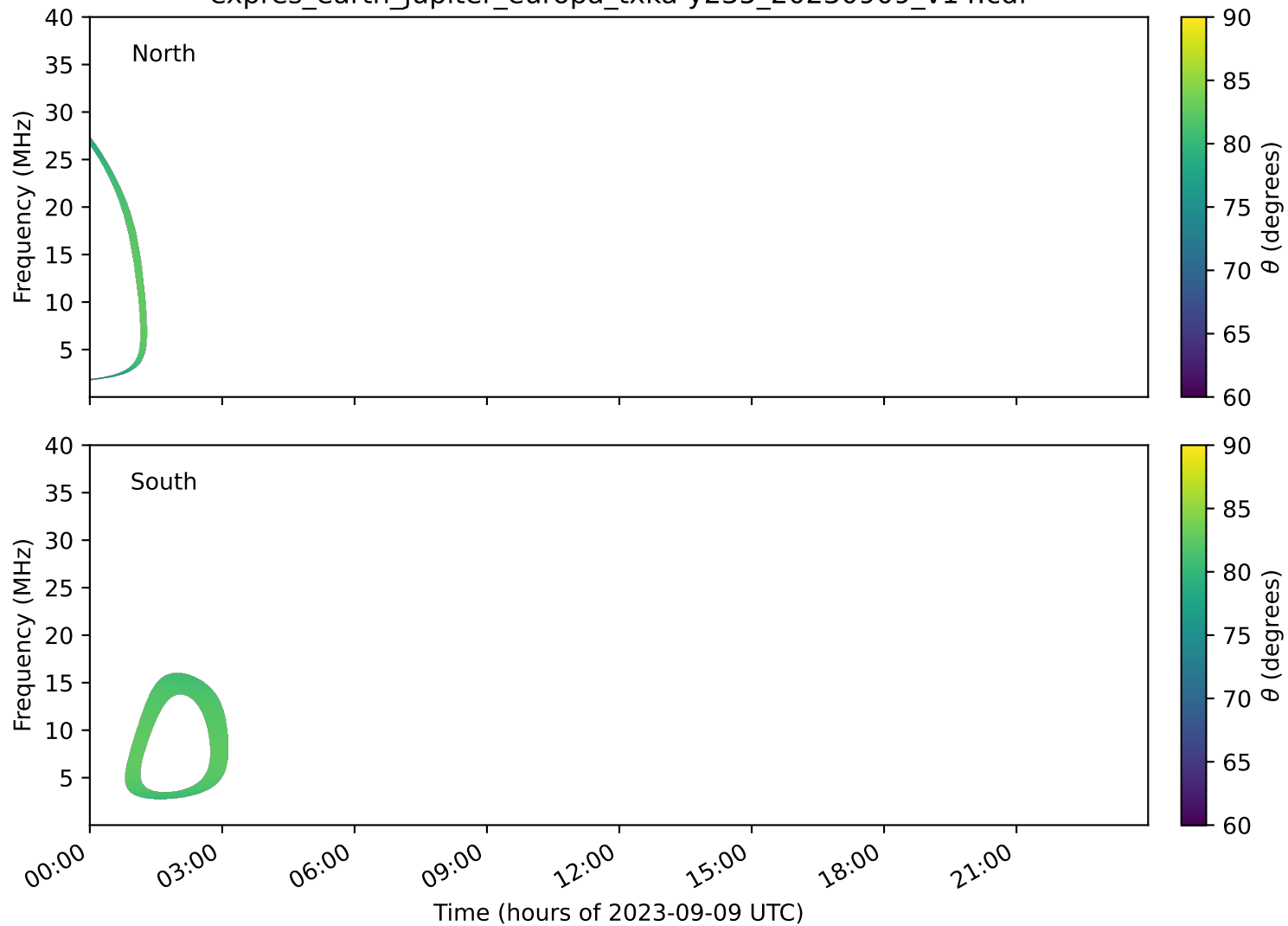
expres_earth_jupiter_europa_txka-y235_20230909_v14.cdf
