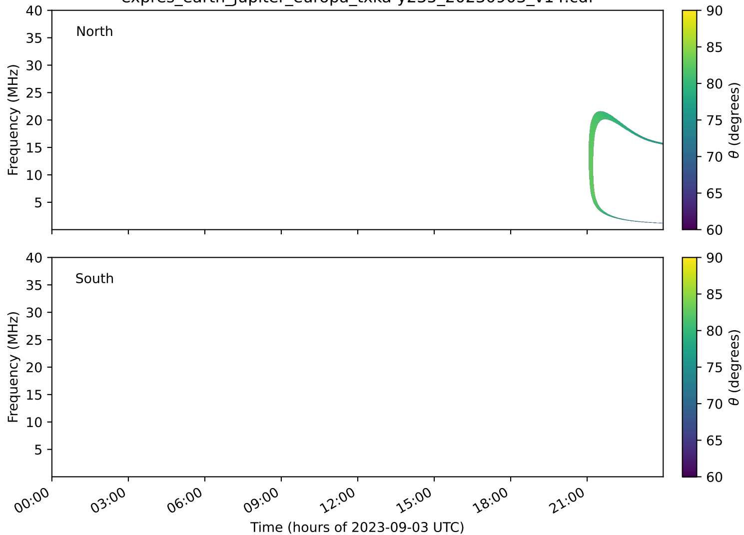
expres_earth_jupiter_europa_txka-y235_20230903_v14.cdf
