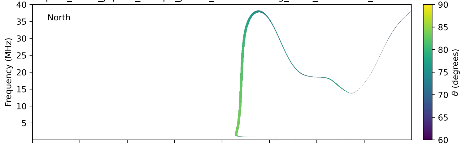
expres_earth_jupiter_europa_jrm33_lossc-wid1deg_3kev_20230907_v11.cdf
