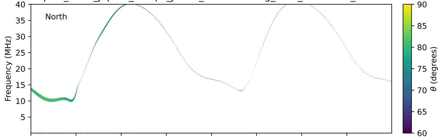
expres_earth_jupiter_europa_jrm09_lossc-wid1deg_3kev_20230904_v11.cdf
