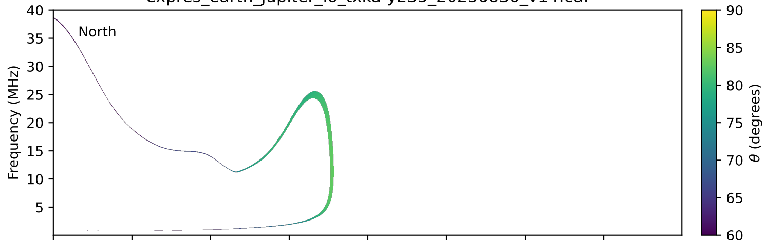
expres_earth_jupiter_io_txka-y235_20230830_v14.cdf
