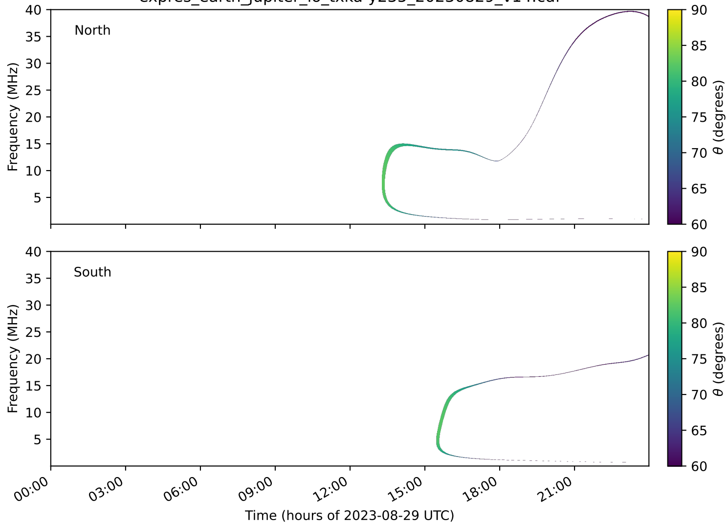
expres_earth_jupiter_io_txka-y235_20230829_v14.cdf
