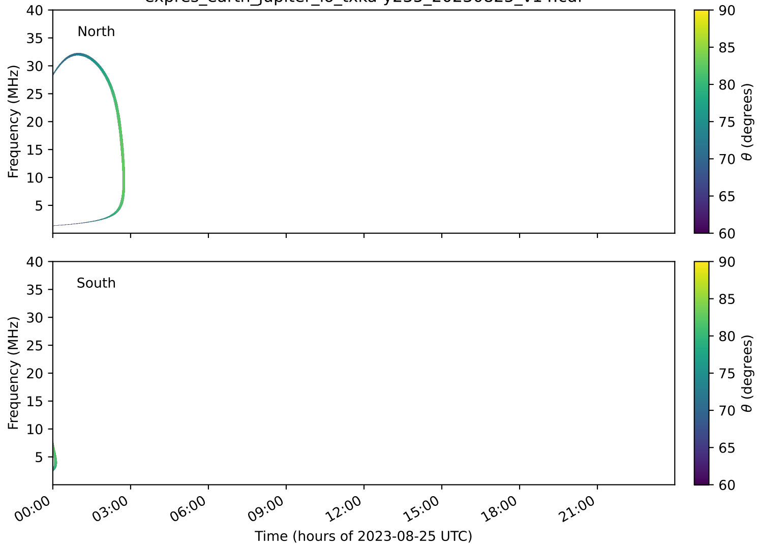
expres_earth_jupiter_io_txka-y235_20230825_v14.cdf
