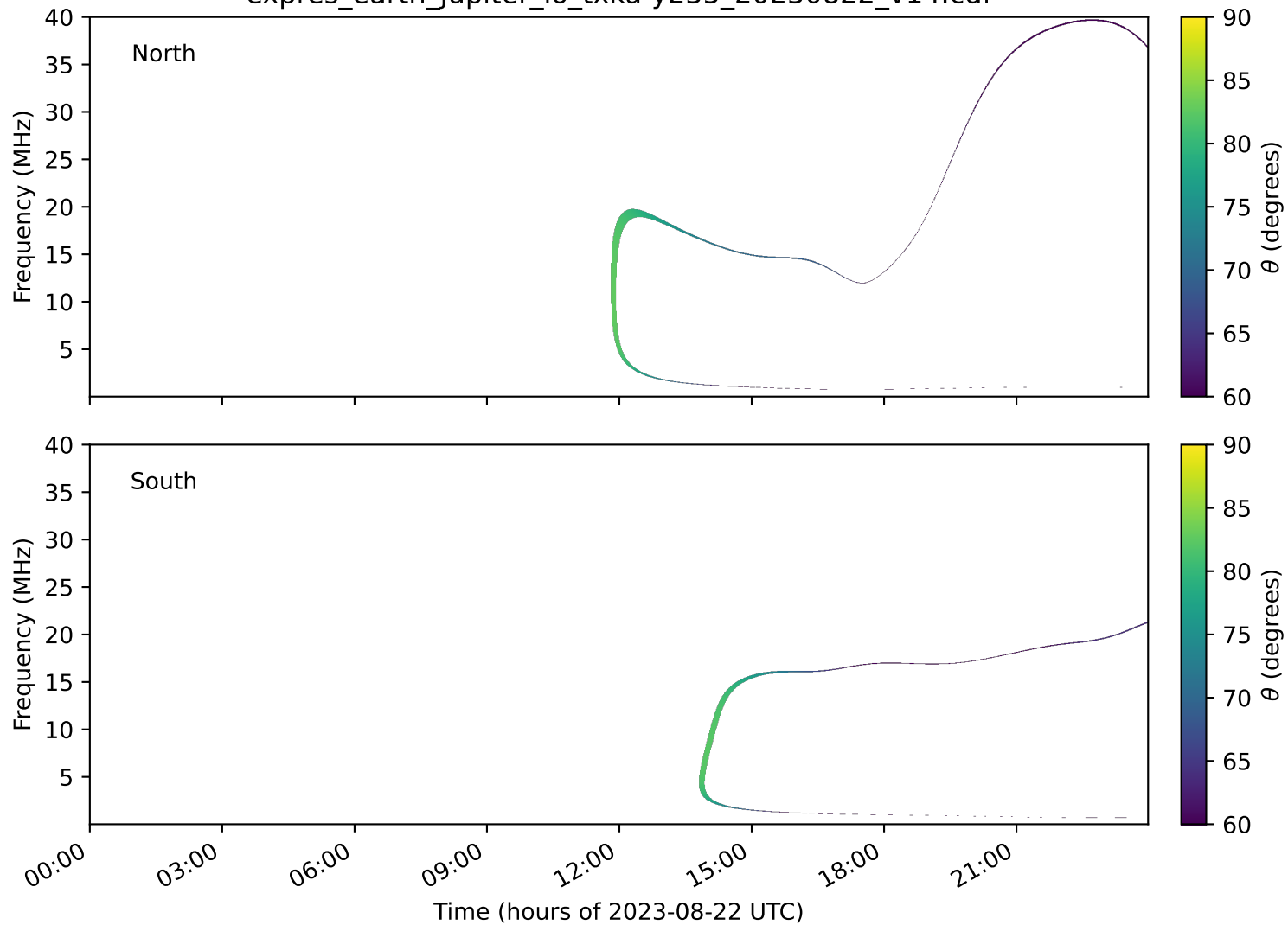
expres_earth_jupiter_io_txka-y235_20230822_v14.cdf
