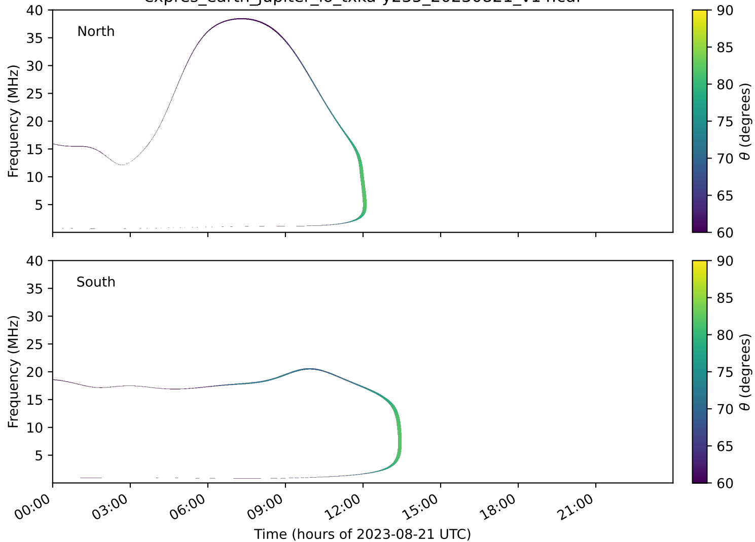
expres_earth_jupiter_io_txka-y235_20230821_v14.cdf
