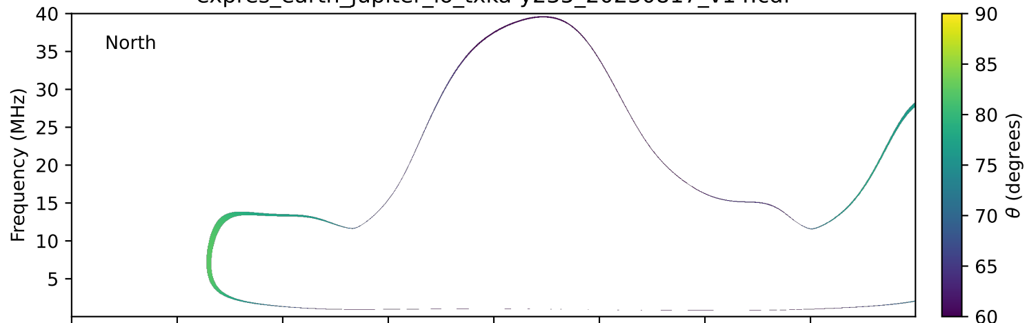
expres_earth_jupiter_io_txka-y235_20230817_v14.cdf
