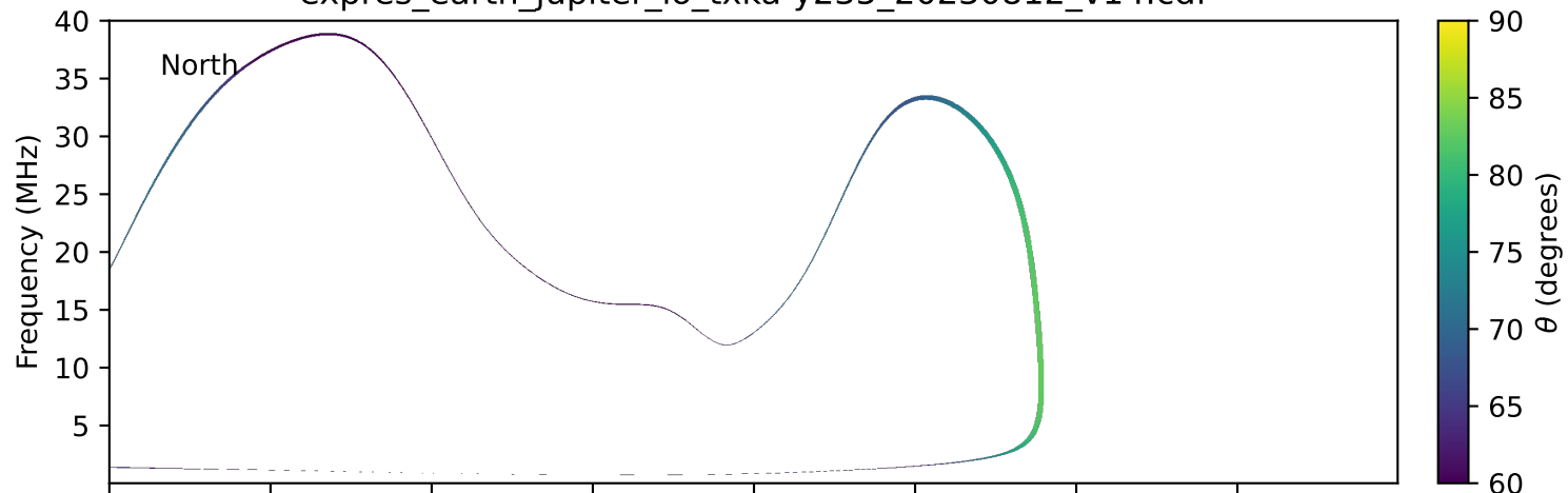
expres_earth_jupiter_io_txka-y235_20230812_v14.cdf
