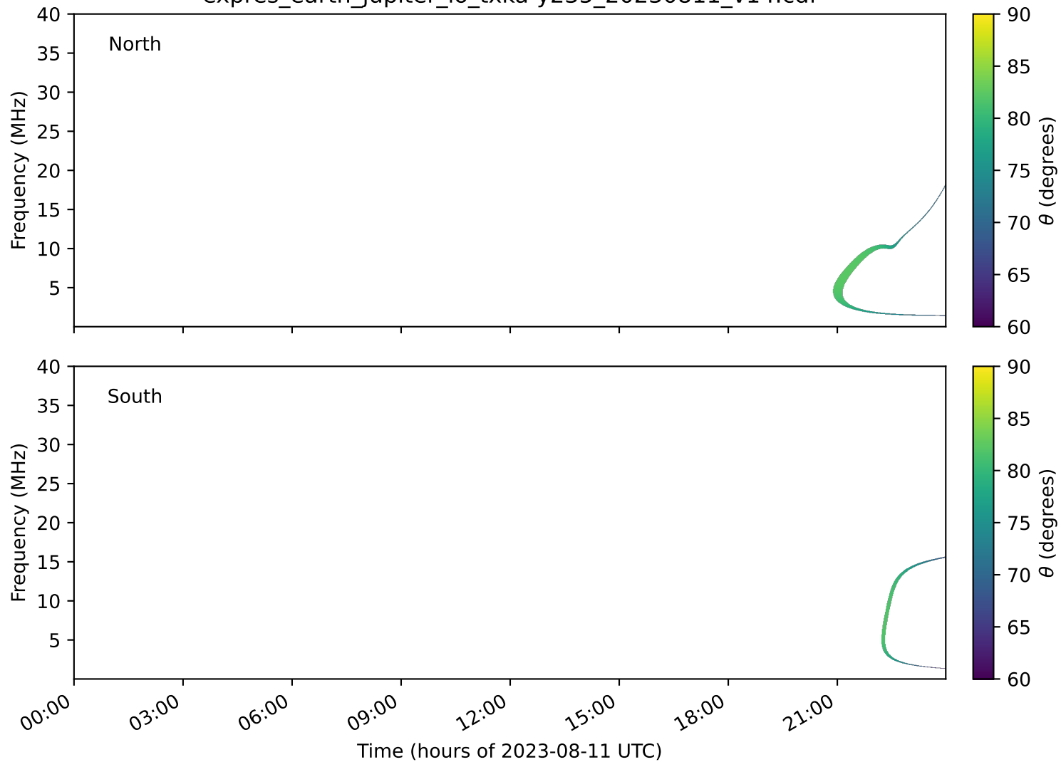
expres_earth_jupiter_io_txka-y235_20230811_v14.cdf
