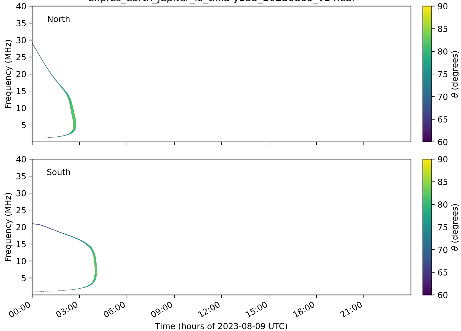
expres_earth_jupiter_io_txka-y235_20230809_v14.cdf
