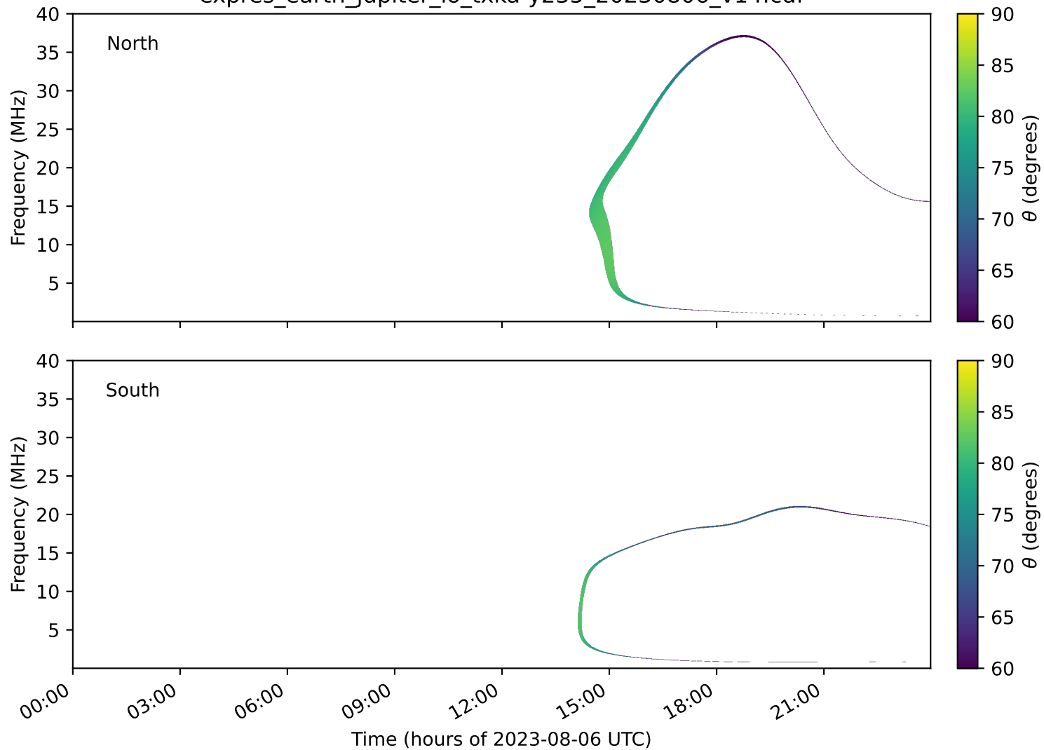
expres_earth_jupiter_io_txka-y235_20230806_v14.cdf
