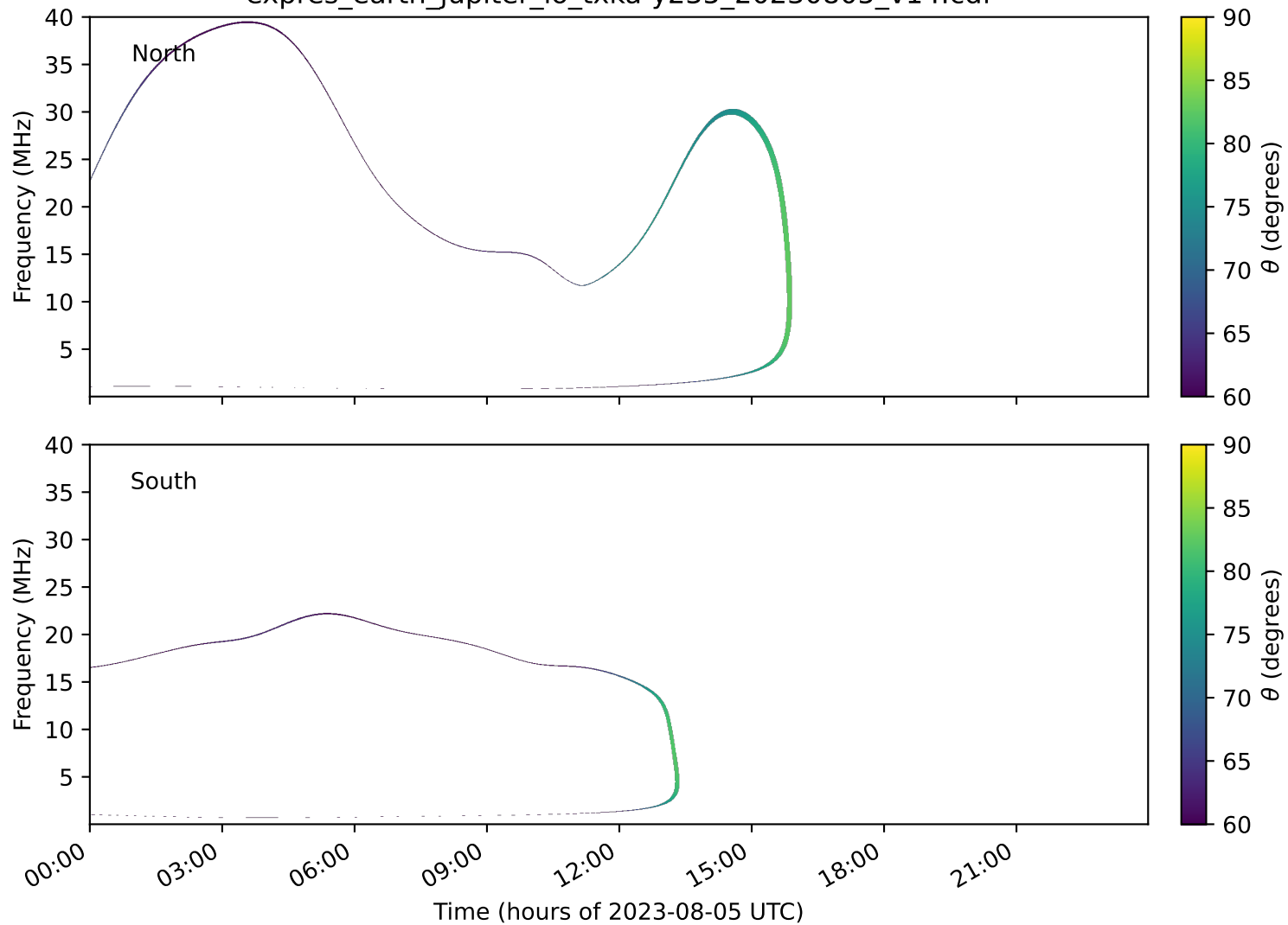
expres_earth_jupiter_io_txka-y235_20230805_v14.cdf
