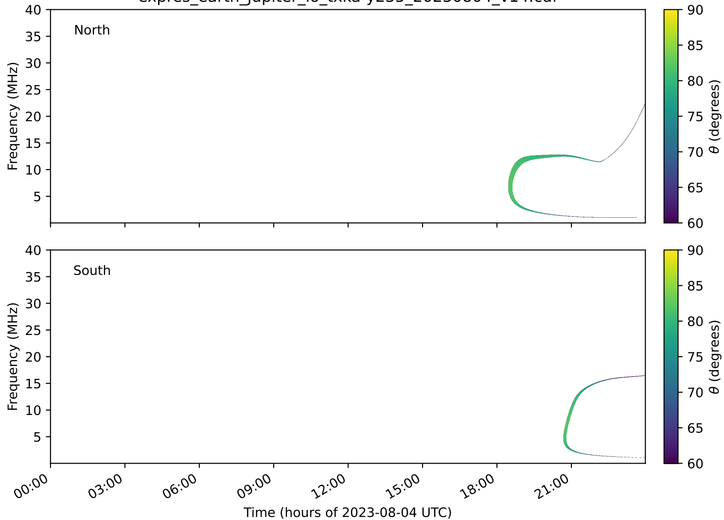
expres_earth_jupiter_io_txka-y235_20230804_v14.cdf
