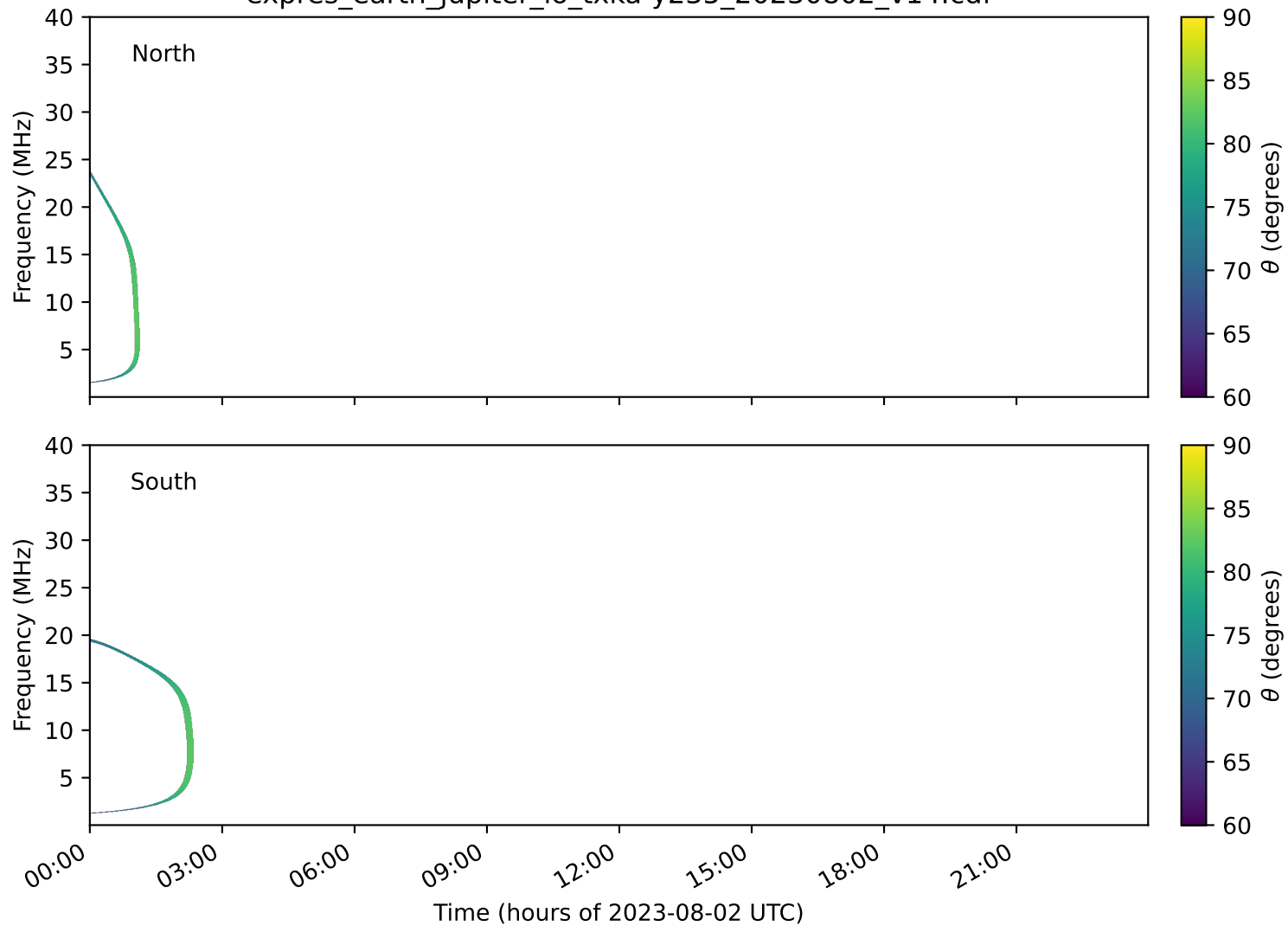
expres_earth_jupiter_io_txka-y235_20230802_v14.cdf
