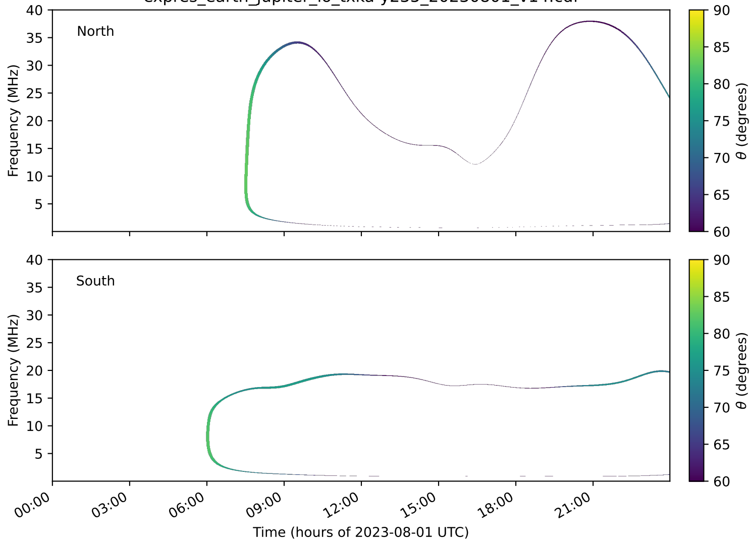
expres_earth_jupiter_io_txka-y235_20230801_v14.cdf
