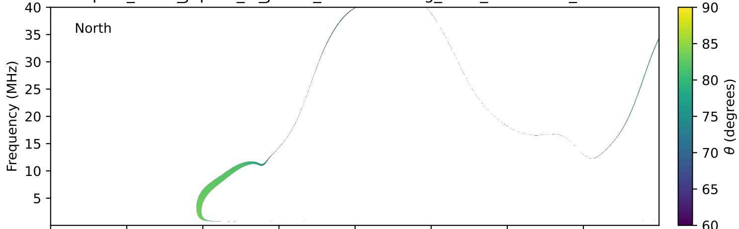
expres_earth_jupiter_io_jrm33_lossc-wid1deg_3kev_20230824_v11.cdf
